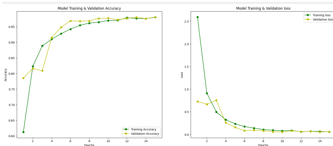
Fig.3 Training and validation accuracy increase steadily while loss decreases, indicating effective learning and good model generalization ( CNN classifiers ).
